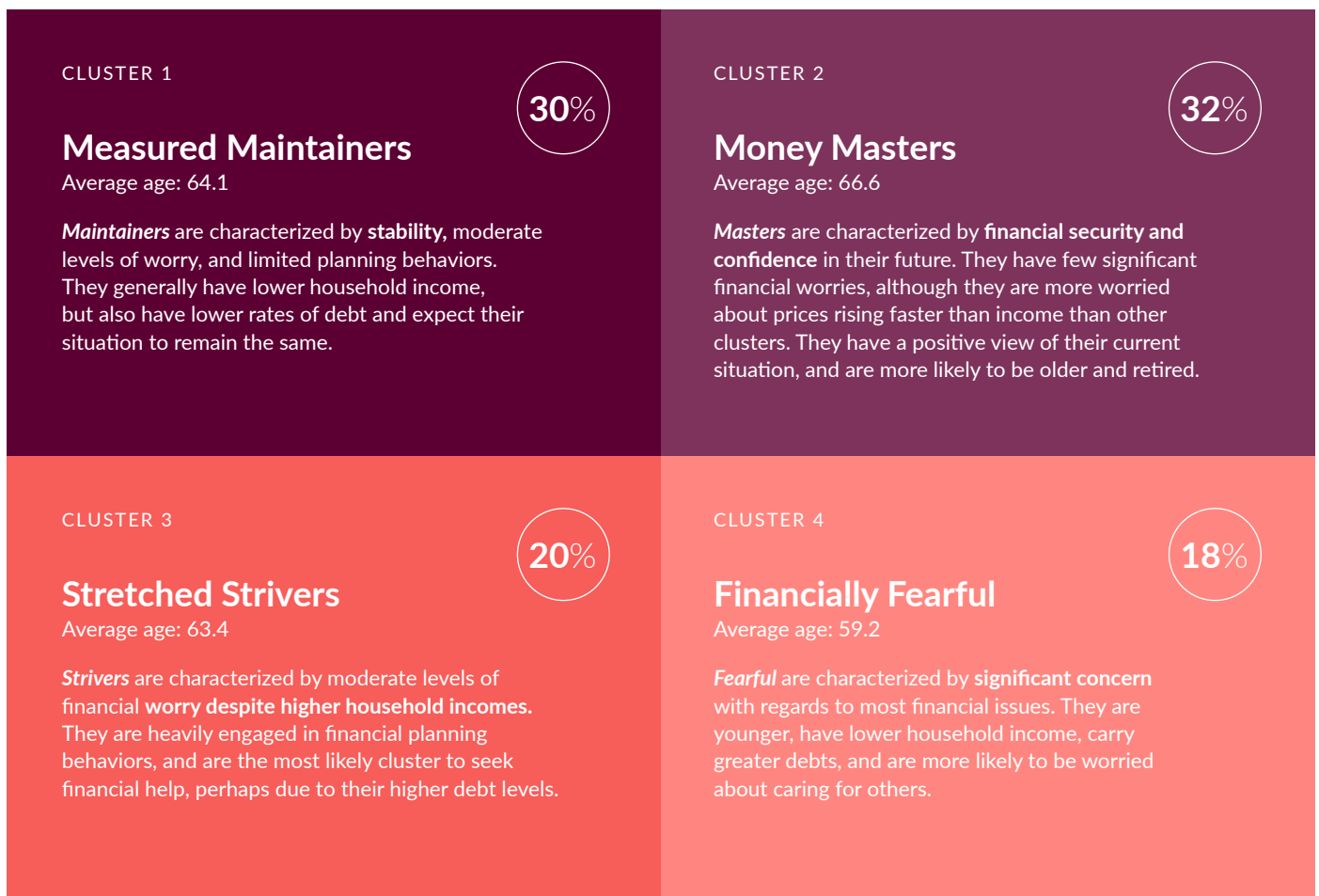
Figure 2: Cluster Descriptions
